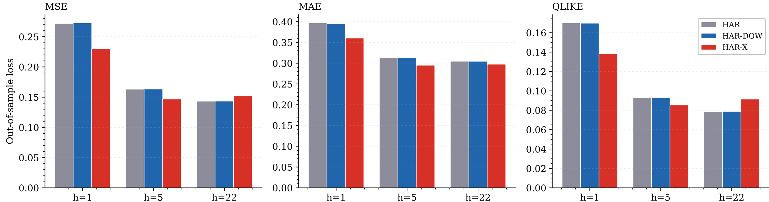
Out-of-sample loss by model and horizon (test 2024+)
